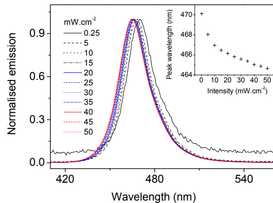
Figure 1: Blue LED (NICHIA NSPB 500S) emission spectra measured during linear ramping from 0 to 50 \text{mW.cm}^{-2} in 600 s. The emission is achieved using four blue LED clusters in the Risø stimulation head, with each cluster consisting of seven LEDs and a 2.5 mm thick Schott GG-420 at the front. The spectra were recorded using a symmetrical crossed Czerny-Turner imaging spectrometer with a focal length of 101 mm, slit width of 25 microns, a ruled grating with a density of 300 lines/mm. The spectrometer, a QE65000 from Ocean Optics, is equipped with a Hamamatsu S7031-1006 FFT-CCD back-thinned detector.
